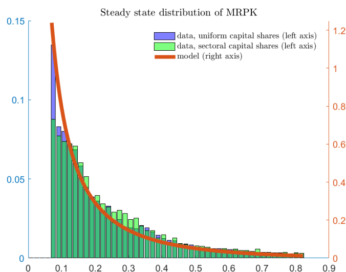
Figure 10: MRPK distribution
