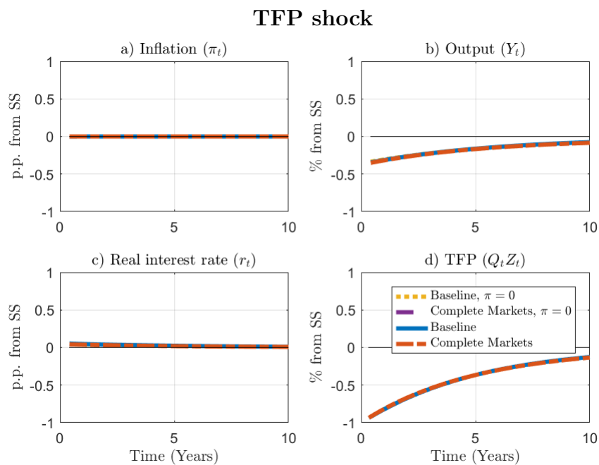
Figure 15: Timeless Ramsey policy in response to other shocks
